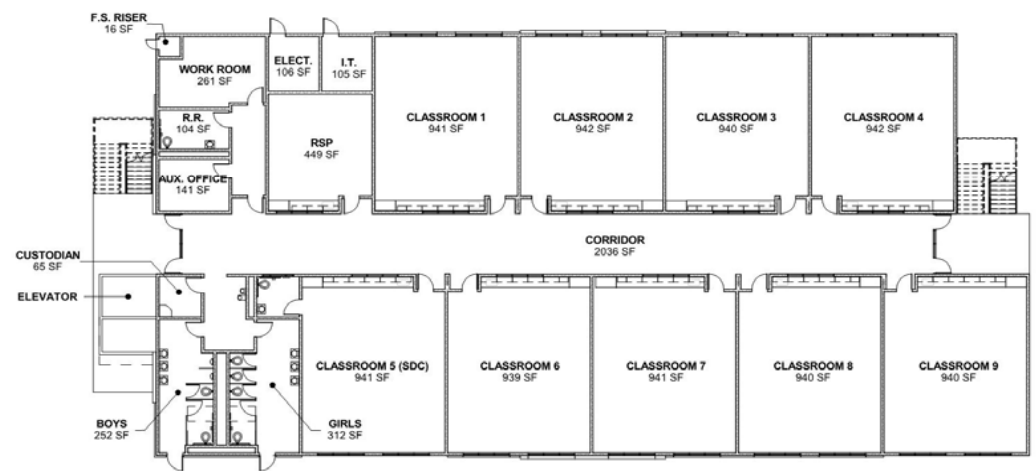
TWO STORY CLASSROOM FIRST FLOOR PLAN
